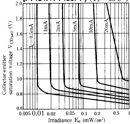
Fig.9-b Collector-emitter Saturation Voltage vs. Irradiance (PT481F/PT483F1) ( T_a = 25^\circ\text{C} )
