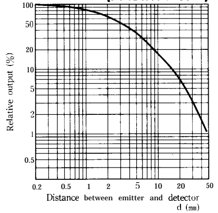
Fig.10 Relative Output vs. Distance (Emitter : GL480) (PT481F/PT483F1)
